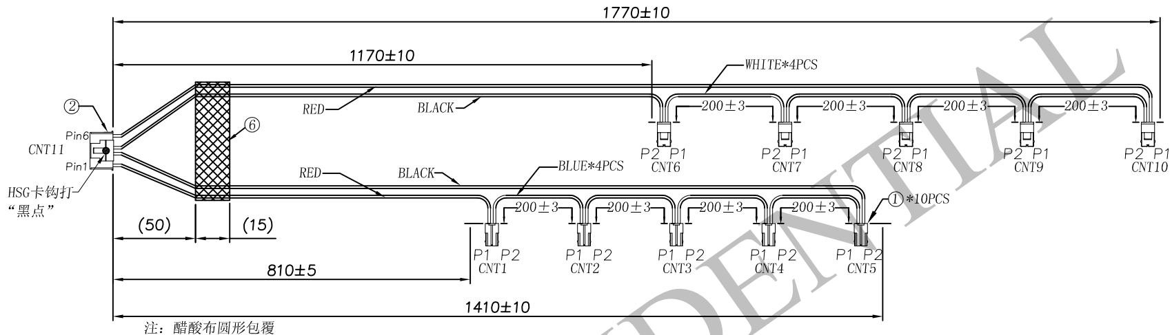
<Pin Assignment>
