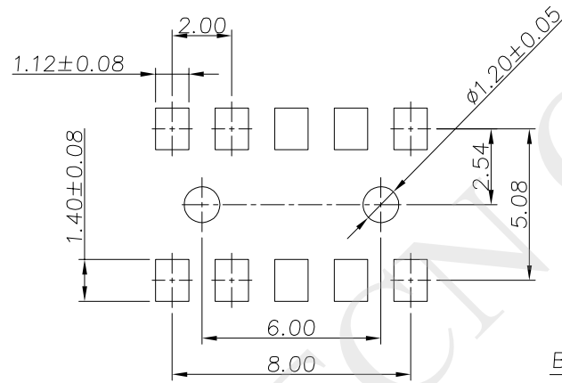
P.C.B LAYOUT GENERAL TOLERANCE ±0.05
